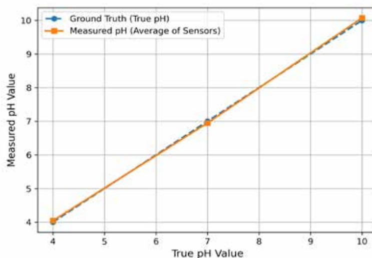
Ground truth validation of pH sensors
